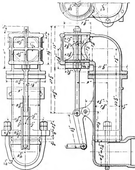
Figs. 3070-3072. Throttle Valve for Ten-Wheel (1-6-0) Locomotive Plant System.
